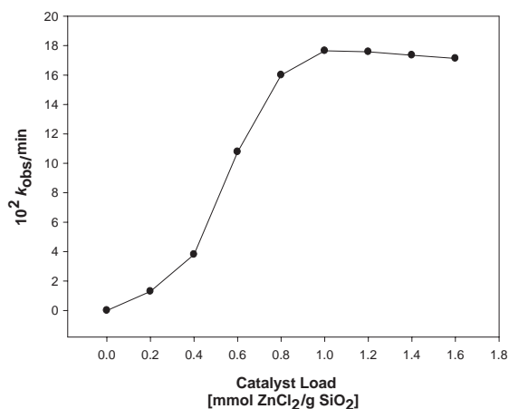
Figure 2. k_{\text{obs}} for the alcoholysis of paraoxon as a function of catalyst load.
